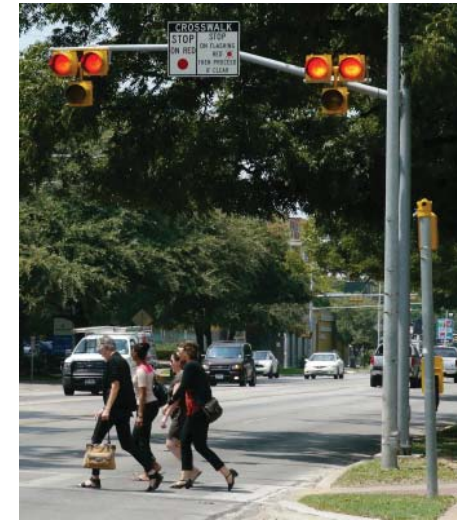
PEDESTRIAN HYBRID BEACON (SOURCE: KXAN , TEXAS)
